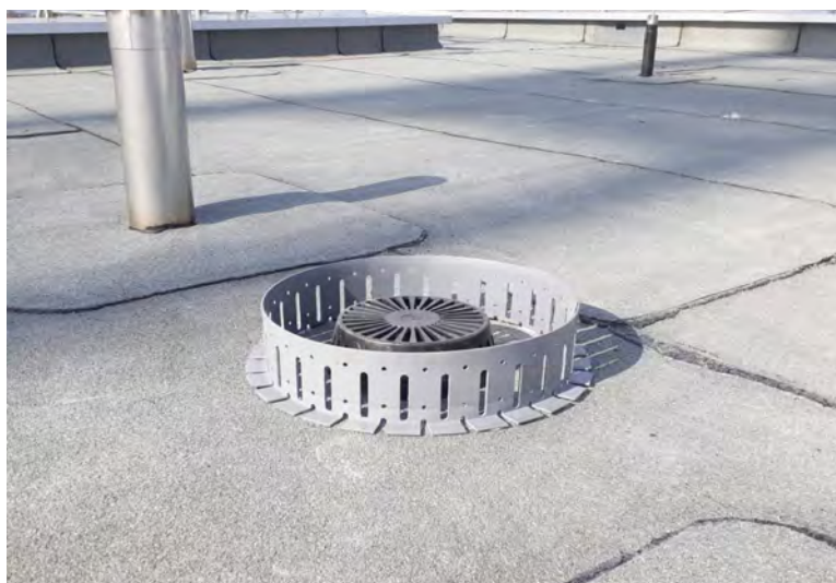
The gravel ring made of robust PVC efficiently retains the roof gravel.
